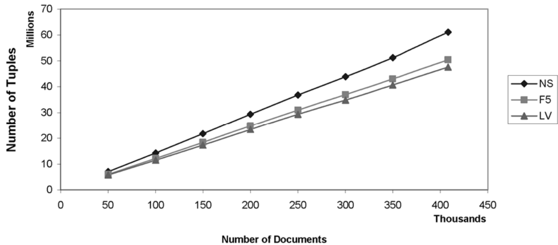
FIG. 4. Number of posting list tuples vs. collection size.
