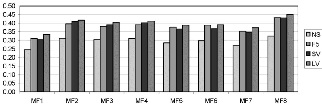
FIG. 2. Bpref values of NS, F5, SV, and LV with matching functions MF1-MF8 using Q_M .
