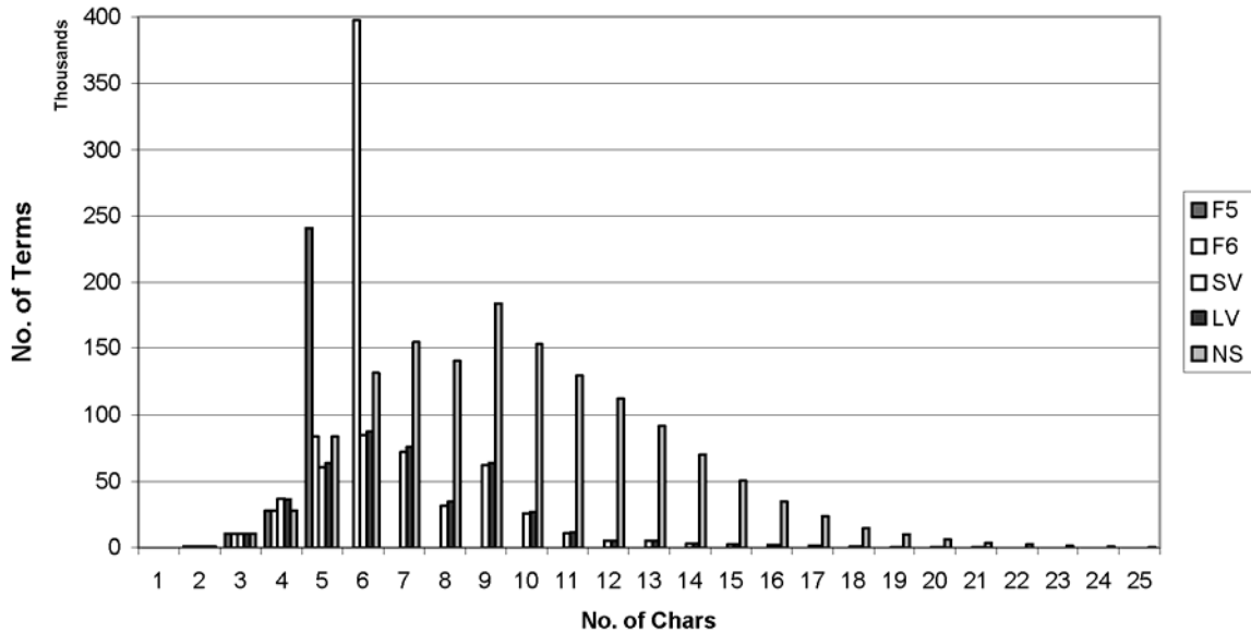
FIG. 1. Term frequency vs. term length (in characters) for all stemmers.
