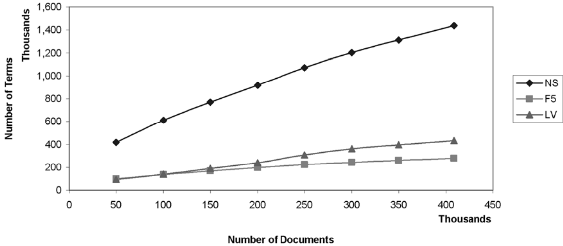
FIG. 3. Indexing vocabulary size vs. collection size.
