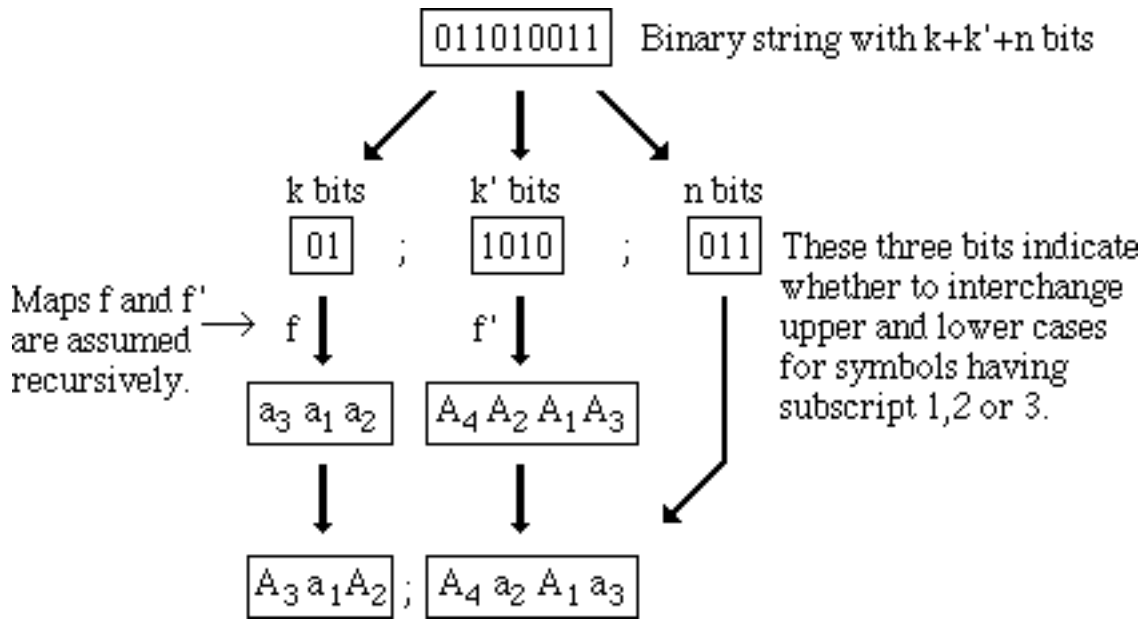
Figure 4: The construction of an embedding f':Q(k+k'+n) \subseteq \text{TranS}(n+n') from assumed embeddings f:Q(k) \subseteq \text{TranS}(n) and f':Q(k') \subseteq \text{TranS}(n')
